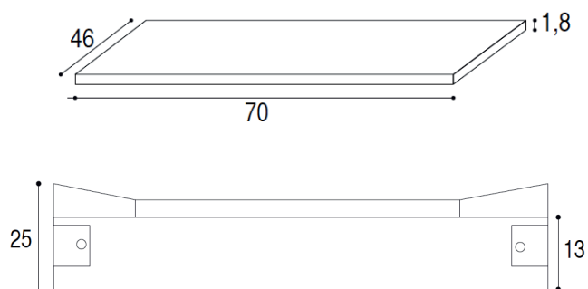
KL45/70H25C
