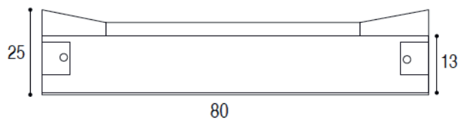
KL24/60H60A
