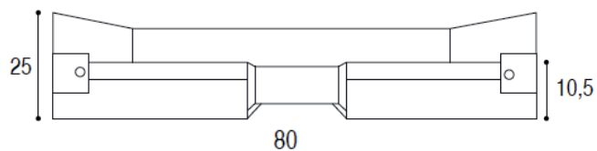
KL45/80H25CS
